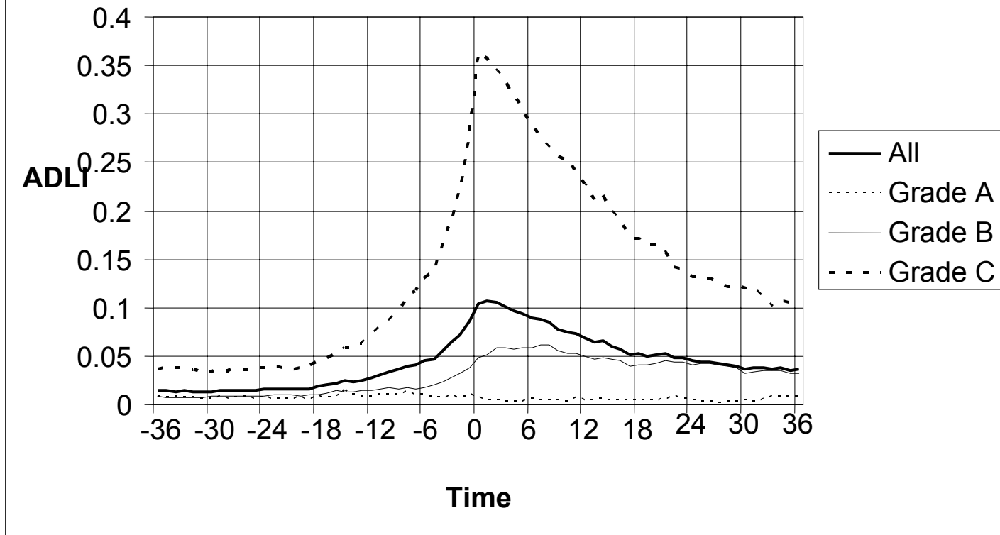
Figure 1: Average DLI around Downgrades
