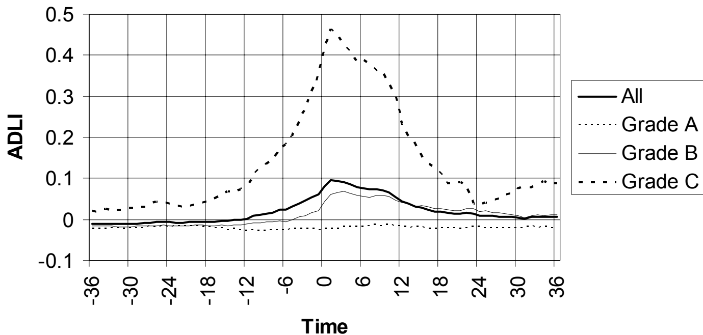
Figure 2: Average DLI (Orthogonalized) around Downgrade
